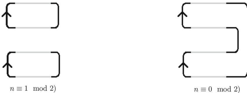
Fig. 4 Positive orientation on a 2-component rational link
