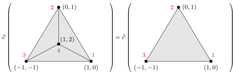
Fig. 3 Two simplicial chains with vector functions having the same boundary
