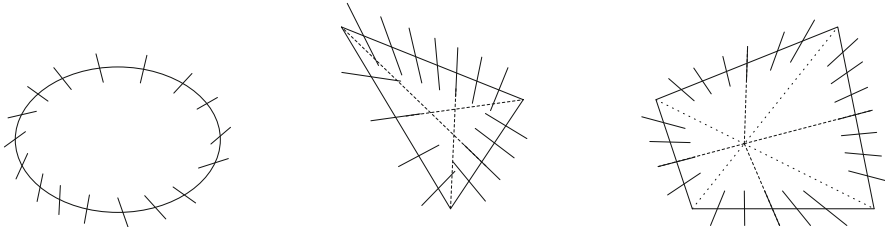
Fig. 3 Left: a convex closed curve with a field of transverse lines. Center: the so-called right-spherical billiard which is 3-reflective. It is defined by triangular domain, and each transverse line on a side join the opposite vertex of the triangle. Right: a 4-reflective projective billiard inside a quadrilateral. The transverse lines join the intersection point of the latter's diagonals
