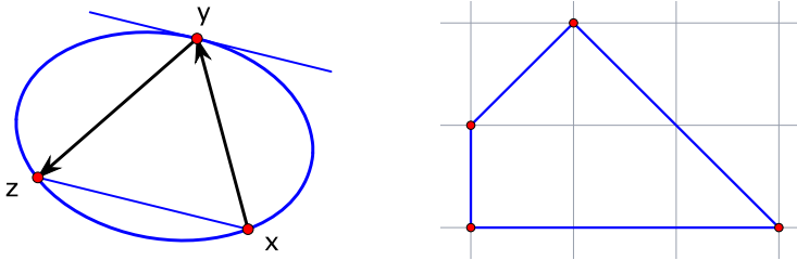
Fig. 7 Left: the chord xy reflects to yz if the tangent line to the oval at y is parallel to xz . Right: all orbits in this quadrilateral are periodic (with the periods equal to 20 and 36)
