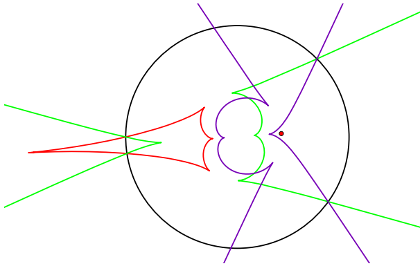
Fig. 8 The first three caustics by reflection in a circle
