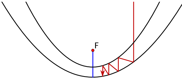
Fig. 5 Trap for a parallel beam of light: F is the focus of the parabolae
